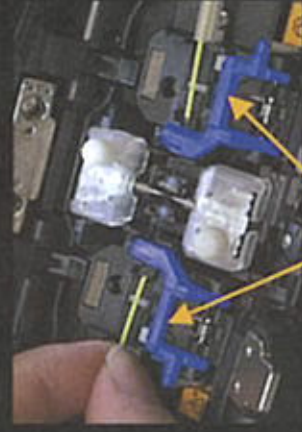
Fiber retention clamps
